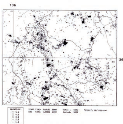
Epicenter for Reihoku Area 2001.01 - 2012.03 (M ≥ 1.0, H ≤ 30km)
